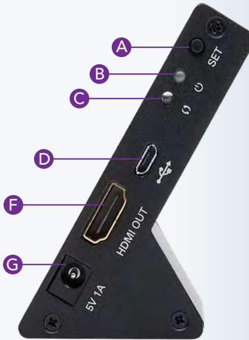
Receiver (Side View)
