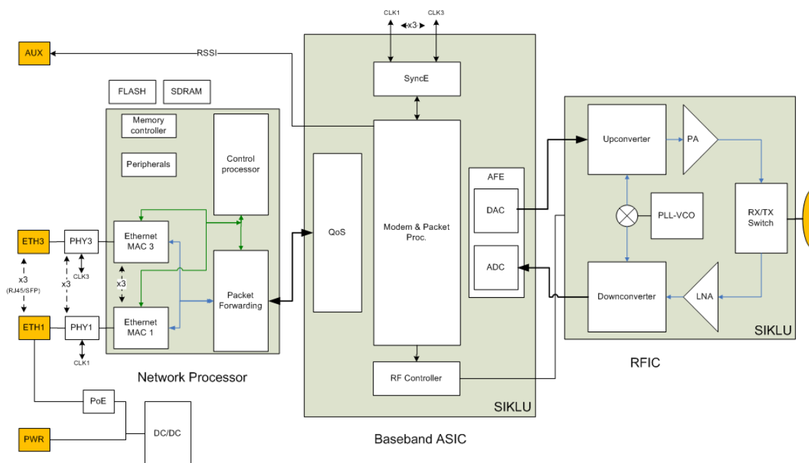
Figure 3 - EtherHaul™ 600T functional block diagram
