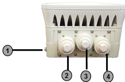
Figure 4 - EtherHaul™ 600T interfaces
