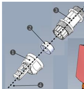
Figure 5 - EtherHaul™ 600T connector gland assembly
