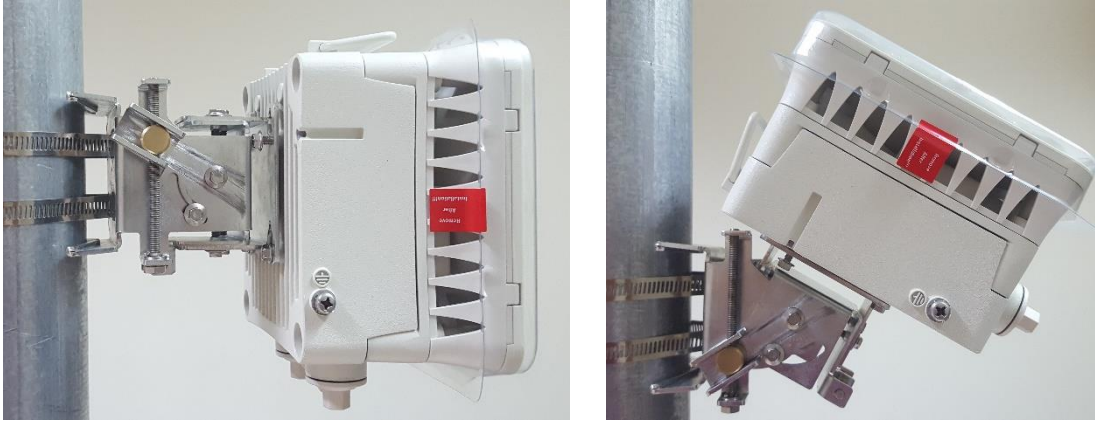
Figure 6 - EH-600T installed
