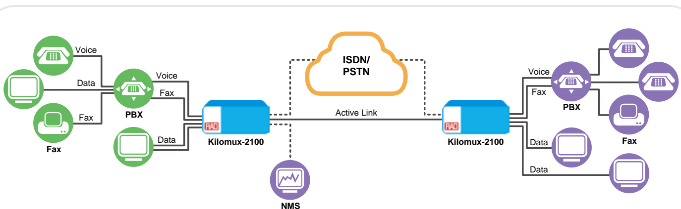
Figure 2. Point-to-point Topology
